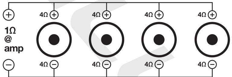
FOUR 4Ω SVC WOOFERS = 1Ω LOAD
