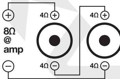
TWO 4Ω SVC WOOFERS = 8Ω LOAD
