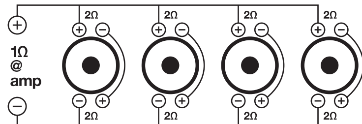
FOUR 2Ω DVC WOOFERS = 1Ω LOAD
