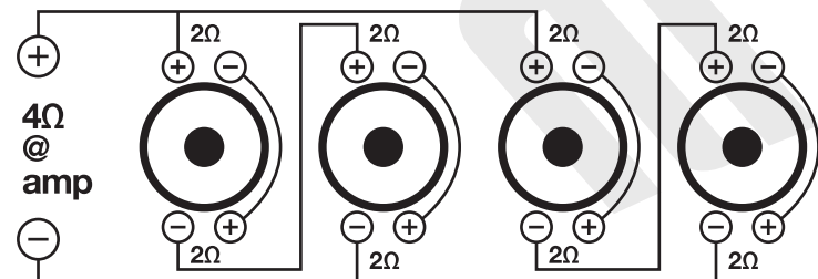
FOUR 2Ω DVC WOOFERS = 4Ω LOAD
